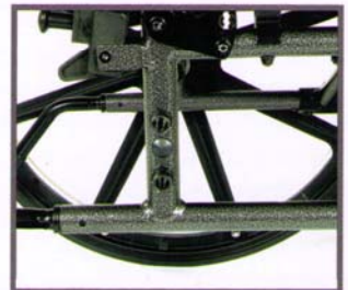
Adjustable Axle Positions Three seat height positions and the ability to add a fixed tilt allow for greater flexibility.
